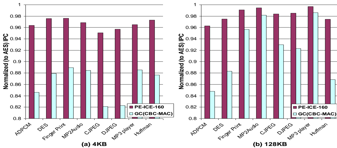
Fig. 12. Run-time overhead of GC, of the AES-ECB engine and of PE-ICE-160 for two data cache sizes (4KB and 128KB)
