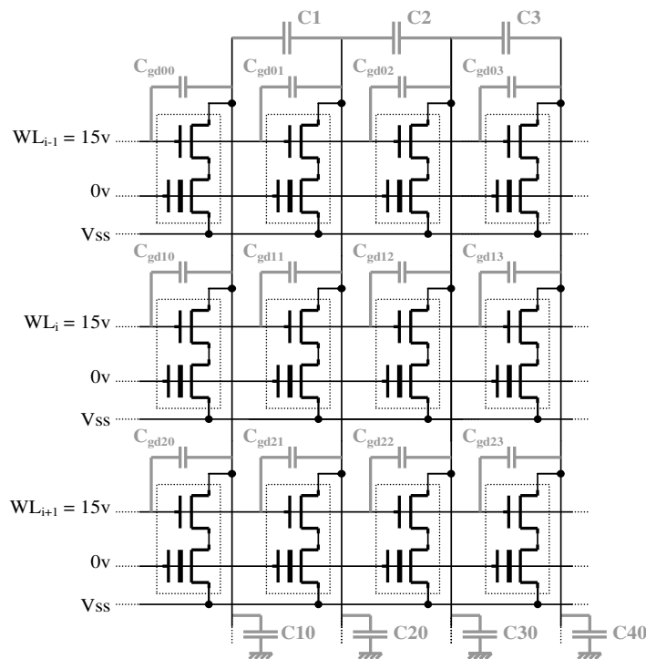
Figure 4.5: Equivalent core cells array in parallel selection
