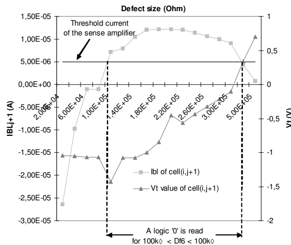
Figure 3.12: VT and I_{BL} of cell(i,j+1) function of Df6 size after a write operation on cell(i,j)
