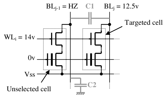
Figure 3.1: Couplage inter bit lines
