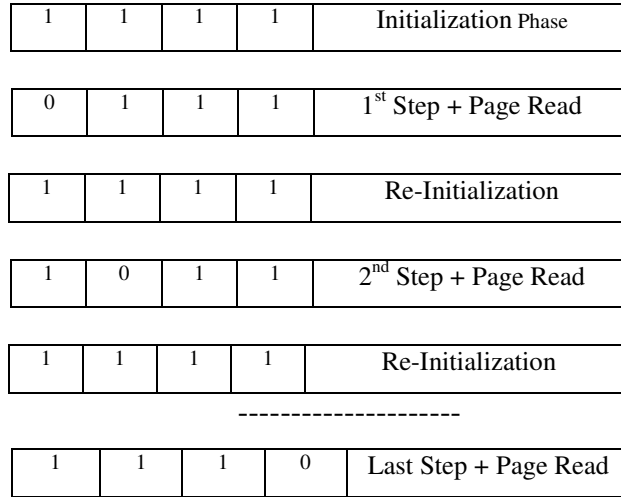
Figure 4.3: SCF(0,0)* exhaustive test approach
