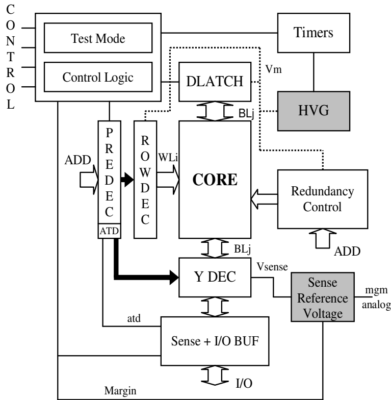
Figure 1.11: Functional scheme of eFlash memories
