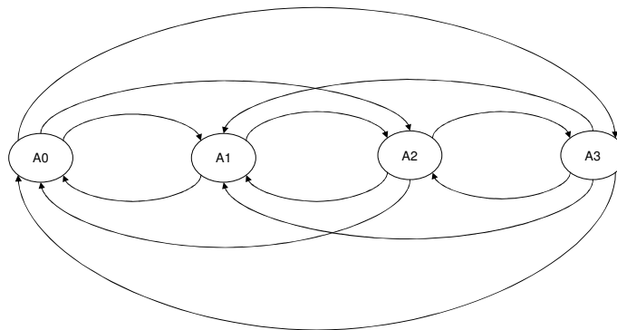
Figure 5.7: State diagram of possible MA_AFs involving four addresses
