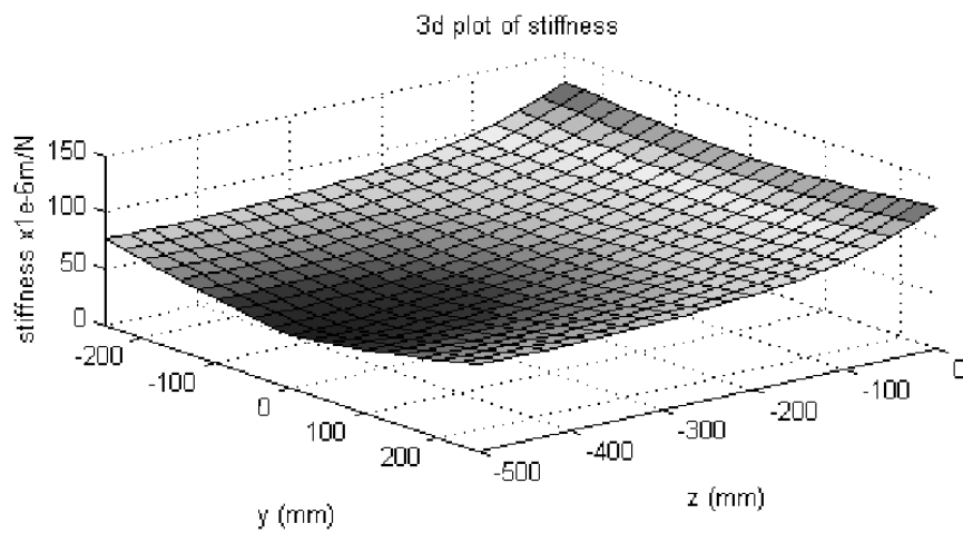
Fig. 6: Stiffness plot
