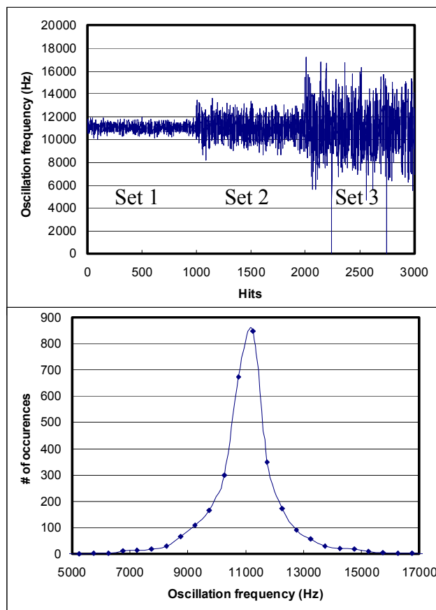
Figure 3: Monte-carlo simulations of the closed-loop system : evolution of the oscillation frequency on 3000 hits (top) and Gaussian distribution of the oscillation frequency (bottom).
