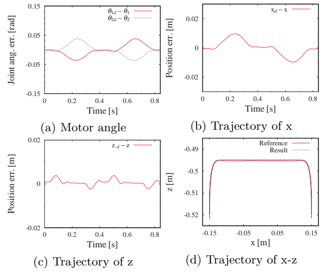
Figure 11: Dynamic control
