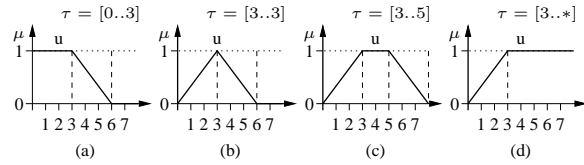
Figure 3: Fuzzy measure of the “certainly” set for \gamma -unexpectedness.
