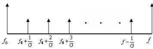
Fig. 5. Bandlimited-Multiple FLC [16].
