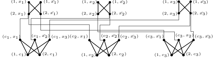
Fig. 5. graph constructed from I_{SAT} = (U, W) with U = \{x_1, x_2, x_3\} and W = \{c_1, c_2, c_3\} with c_1 = \{x_1, \bar{x}_2, x_3\} , c_2 = \{x_1, \bar{x}_2, \bar{x}_3\} and c_3 = \{\bar{x}_1, x_2, \bar{x}_3\} .
