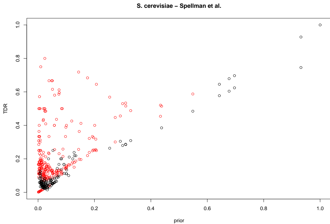
Figure 5 — Gonna performance on yeast. Gonna was applied to the transcriptomic data set published by Spellman et al. (1998) [34] using experimental evidence code annotations only as prior knowledge database. TDRs of all BP GO terms where predictions are proposed by Gonna are plotted as a function of the prior probability of the terms. Red and black points indicate significant and non-significant TDRs , respectively.
