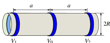
Figure 1: Tripolar electrode cuff model.
