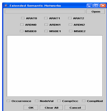
Figure 7: Document classifier
