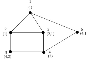
Figure 1: An example of execution of GLS.
