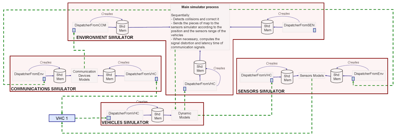
Fig. 2. Detailed view of Thetis. Dashed lines stand for the UDP/IP inter-simulators communications.
