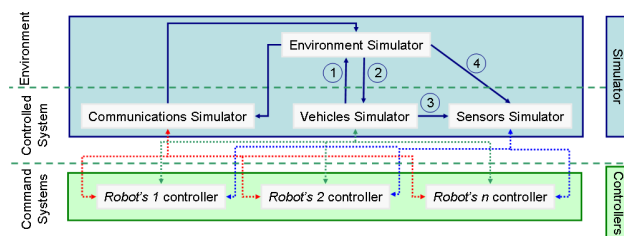
Fig. 1. Simplified architecture of Thetis: there is a logical sequence between 3 simulators even if there are independent processes on different computers. The cycle duration of this sequence must be largely lower than the period of the controller. The temporal decoupling is only effective (and that's enough) between the simulator and the controllers. The link between the communications simulator and the environment simulator is event-driven (when a communication between vehicles occurs).
