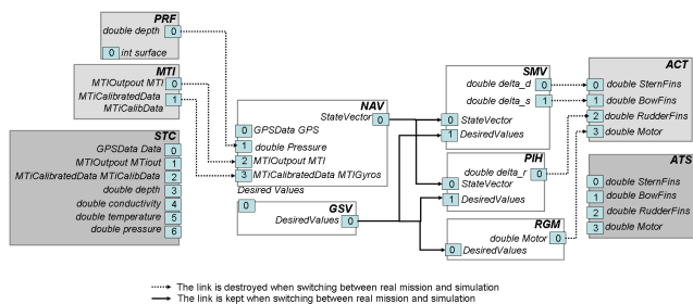
Fig. 4. Connection between the architecture modules
