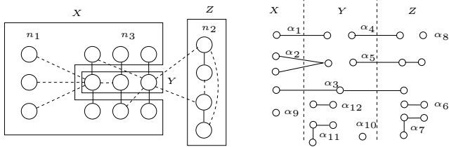
(a) Illustration of the covering of \tau_1
