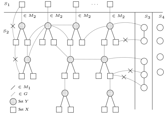
Figure 7. Diagram of the proof of Theorem 2.1
