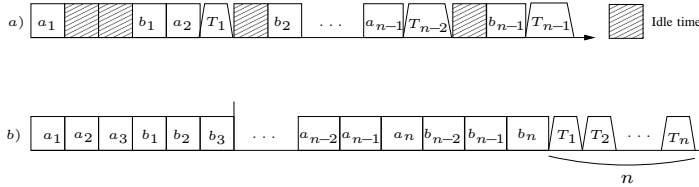
Figure 13. Illustration of the covering of G
