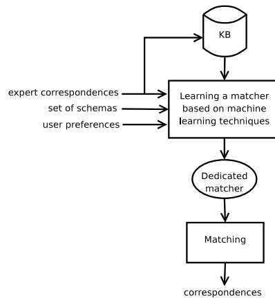
Figure 1: YAM Architecture
