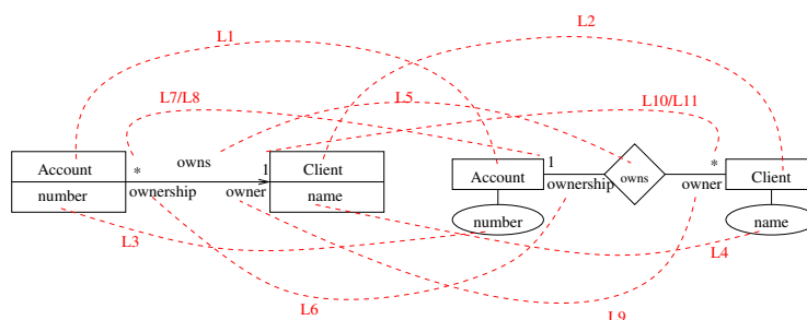
Fig. 2. UML (lhs) and ER (rhs) models in concrete syntax, and transformation links.
