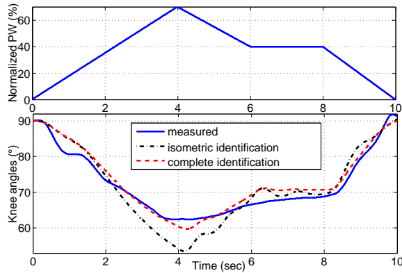
Fig. 4. Pulse Width of stimulation input and the mechanical parameters identification results (The complete model). The isometric model (dash-dot line) is the model before the identification of the mechanical parameters of muscle k_s and K_m .
