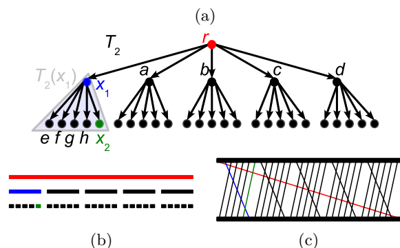
Fig. 1. The interval model (b) and the permutation model (c) of the undirected underlying graph of the transitive closure of the rooted directed tree T_2 (a). This graph has linearity strictly greater than 2, because two orders are not sufficient to represent the closed neighborhood \{r, x_1, x_2\} of x_2 .
