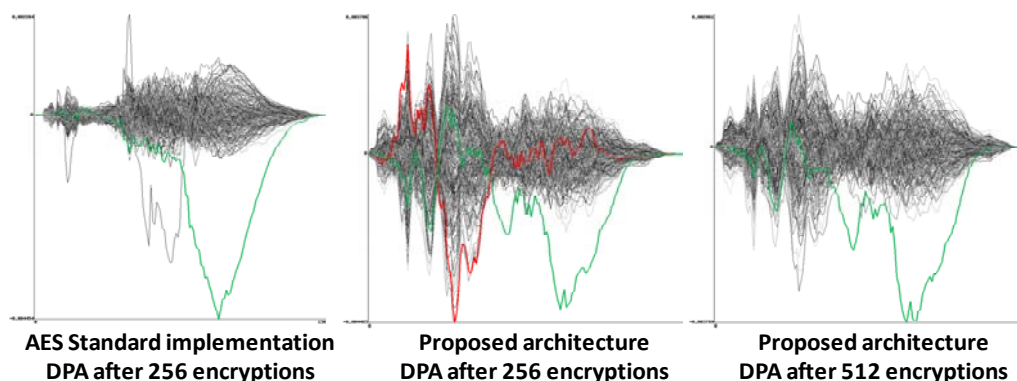
Figure 11: DPA Curves
