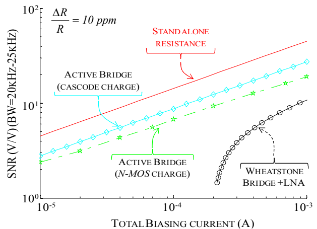
Figure 4. SNR of the active bridge compared to both “ideal” and standard solutions as a function of the current consumption.
