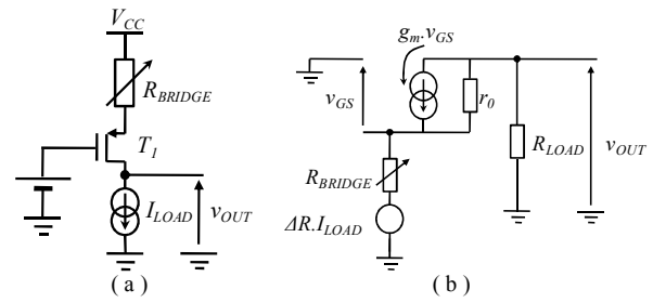
Figure 3. “Active bridge” principle (a) and its small-signal model (b).
