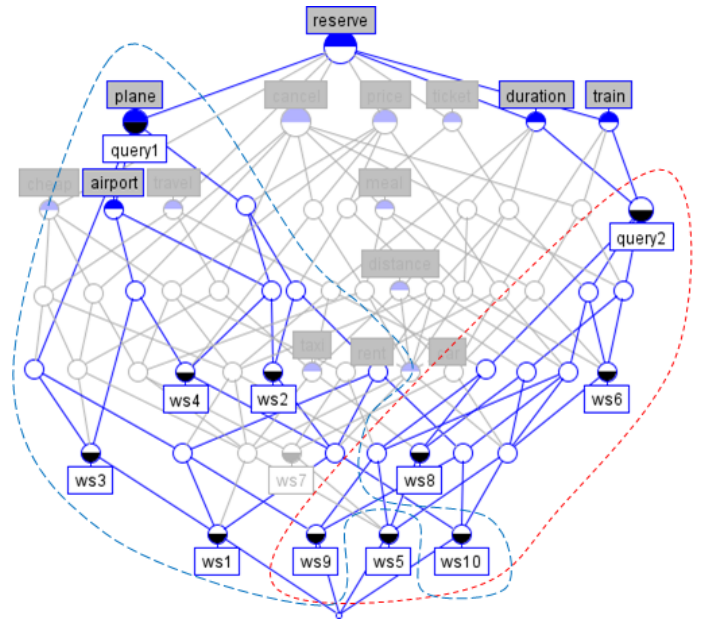
Figure 5. Queries as concepts in the service \times keyword lattice.
