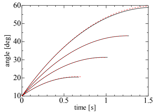
Fig. 11. Dynamic behavior of a swing door when giving several impacts on it.
