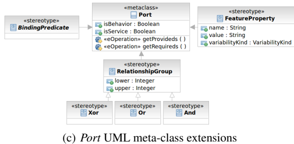
Figure 5 – Meta-classes extensions
