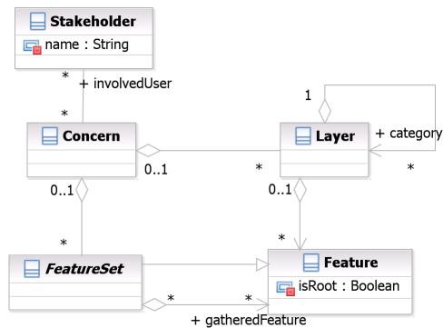
Figure 3 – Feature meta-model excerpt: Layers and feature sets
