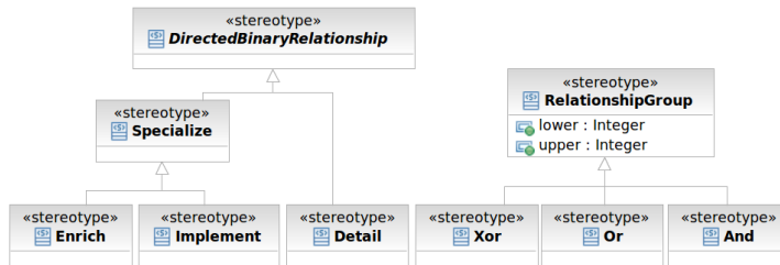
Figure 9 – Feature relationships
