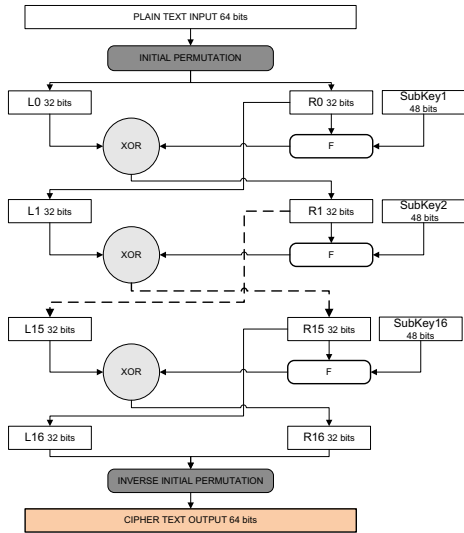
Figure 1. Data Encryption Standard (DES)
