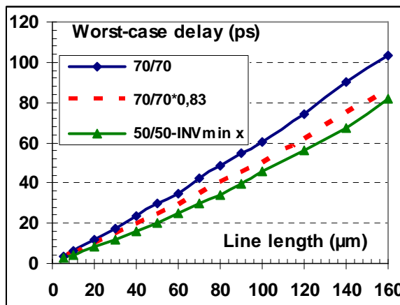
Figure 8: Performance (maximum frequency range and minimum delay) comparison for two different pitches (small lines).
