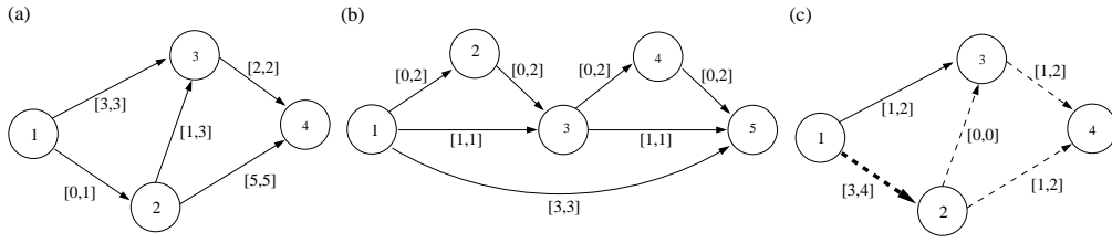
Figure 1: (a) A network in which the necessary criticality of (3,4) cannot be deduced from EST_{34} = LST_{34} (b) A network in which possibly critical activities do not form a possibly critical path (c) Dashed tasks form possibly critical paths, and the bold task is necessarily critical
