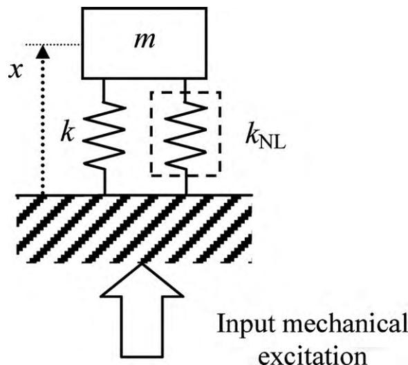
Fig. 1. Equivalent mechanical model for a nonlinear undamped system. Nonlinearity is introduced by an additional nonlinear spring with mechanical stiffness k_{\text{NL}} . The term F_{\text{NL}} is the associated nonlinear force.
