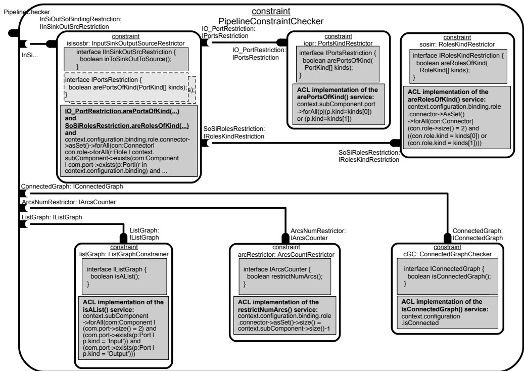
Figure 7: Example of a Constraint-Component Assembly
