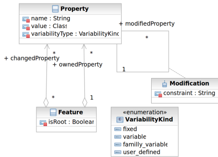
Figure 2. Feature properties
