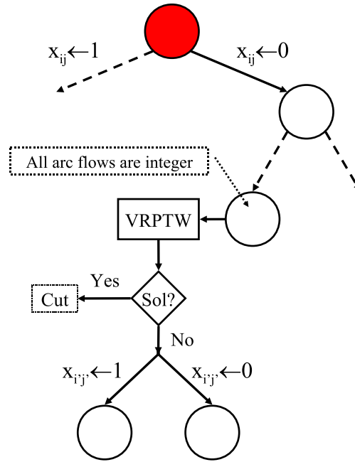
Figure 2: Branching strategy
