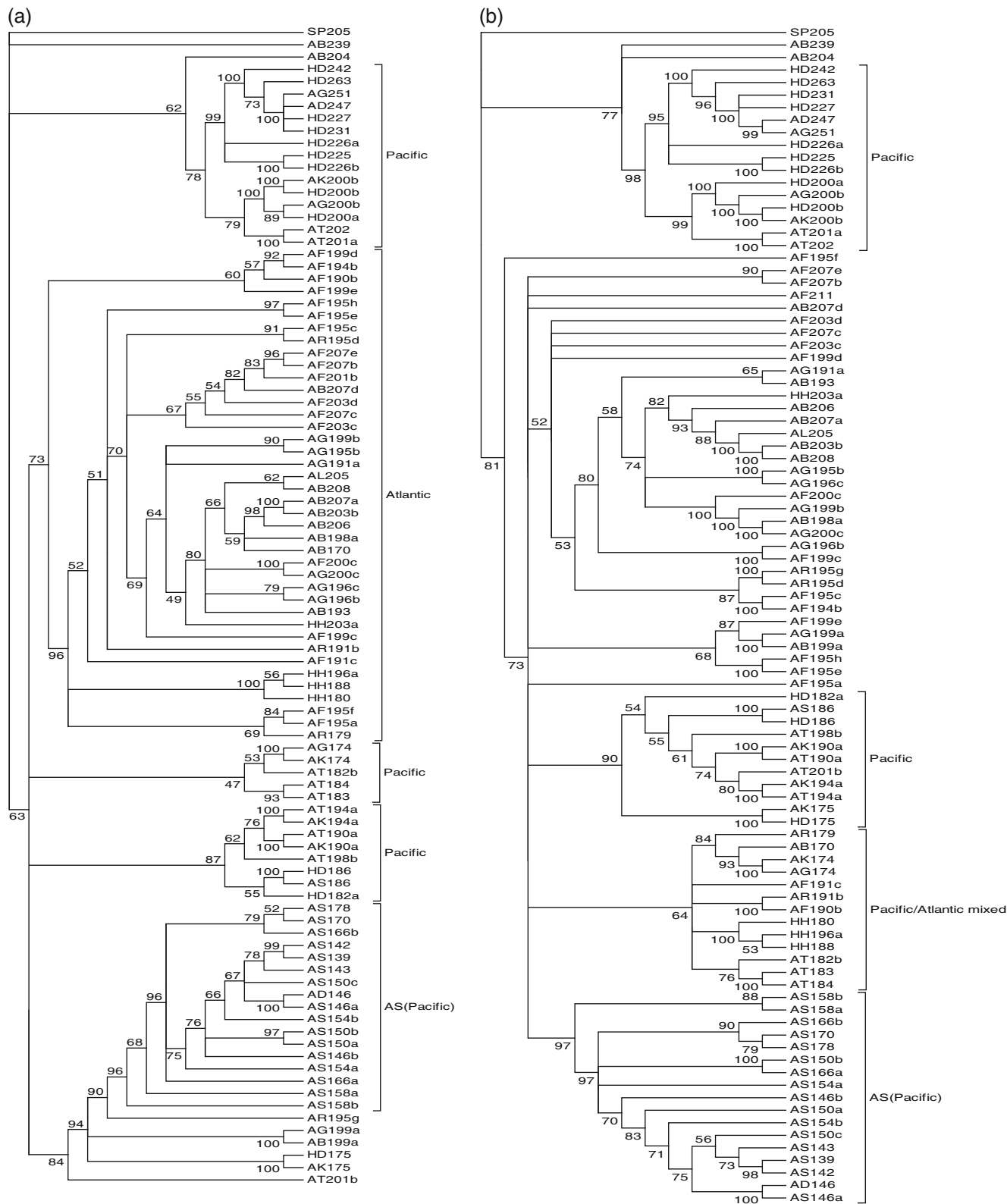
Figure 3. Neighbour-joining trees based on repeat region. (A) Tree I based on repeat region with repeat-like (RL) region. (B) Tree II based on repeat region only. The pairwise molecular divergence among homologous was estimated by aligning their tandem repeat sequences using the MS-Align program (Bérard and Rivals 2003). The tree was inferred with FastME (Desper and Gascuel 2002) from the matrix of pairwise alignment distances. For each internal edge, the confidence value (between 0 and 1) and the rate of elementary well-designed quartets (Re) were computed (Guenoche and Garreta 2000). The abbreviations of the species names are given in table 1.
