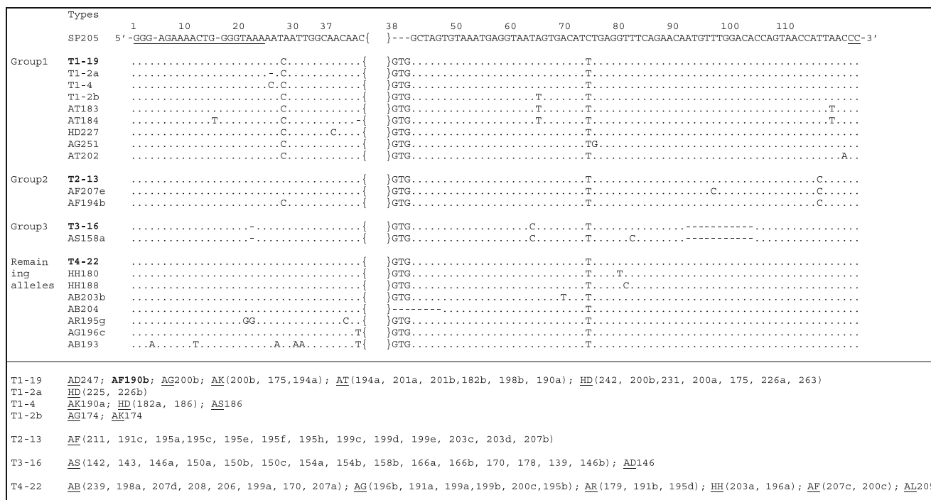
Figure 1. Sequence alignments of 23 haplotypes in the flanking region of locus Spl-106 . The parentheses between position 37 and 38 indicate the repeat region. 5'-primer site is underlined on the left side, while 3'-end primer site is omitted on the right side of this map because no mutations occurred in this primer region. Dots indicate identical sequences. Dashes indicates deletions. The dominant haplotypes were named T1 to T4 with the number of alleles behind them. For example, T4-22 means that the T4 haplotype present in 22 alleles, and the name of these alleles for each haplotype are listed under the alignment map. Rare haplotypes, which is present in only one allele, were named directly with the code of corresponding allele.
