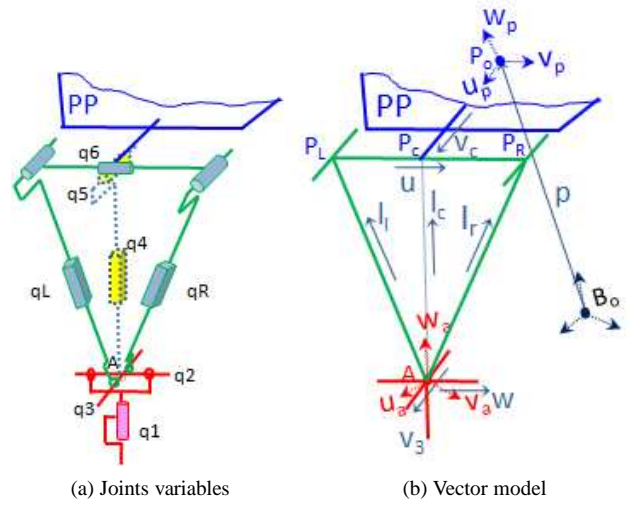
FIGURE 8: CONFIGURATION AND NOTATIONS OF BRANCHES
