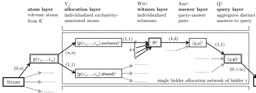
Figure 5: Structure of a Knowledge Allocation Network. Doubly boxed nodes indicate the conservation flow rule, all other internal nodes are multipliers. Edges \langle i, j \rangle are associated with lower bounds and capacities by labels (l_{ij}, c_{ij}) .
