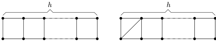
Figure 11: The h -ladder and the h -*ladder.
