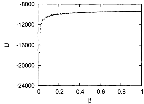
FIGURE 2. Annealing integration under the RAS model for the PGK dataset. The 1,000 values of \ln p(D | \theta, M) sampled during the quasistatic integration are plotted against \beta , shadowing the curve of E_\beta[\ln p(D | \theta, M)] as a function of \beta . The logarithm of the marginal likelihood, as the integral of E_\beta[\ln p(D | \theta, M)] over [0, 1] , can then be estimated as the integral of the curve.
