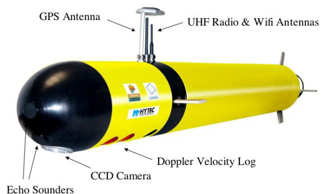
Fig. 1: Sensors equipment (without Sidescan Sonar and CTD Sensor)
