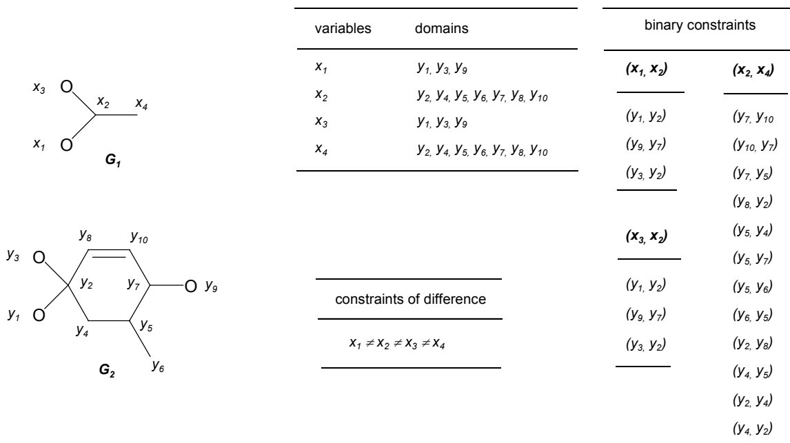
Figure 6. Definition of a CSP to search a matching from graph G_1 to graph G_2 .
