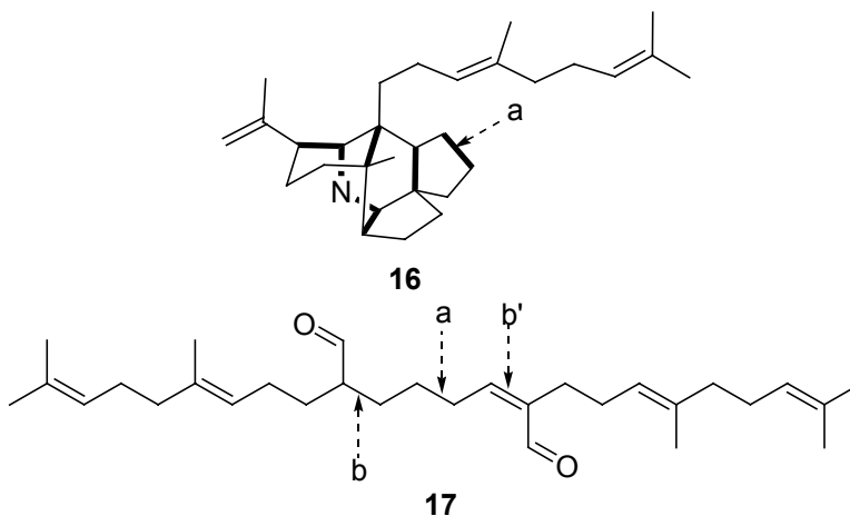
Figure 17. The proto-daphniphylline case.
