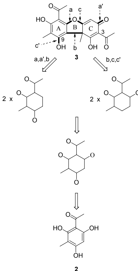
Figure 13. Reflexive analysis of usnic acid.
