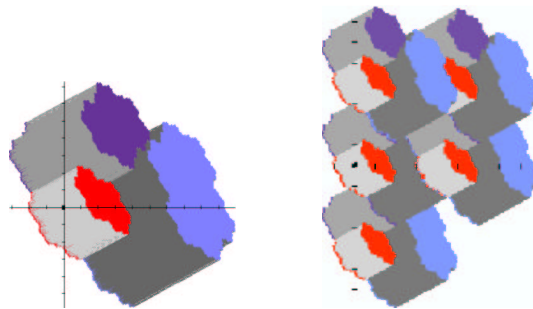
Figure 9: Markov Rauzy fractal; Markov multiple tiling
