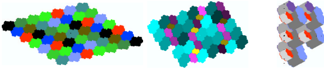
Figure 1: Periodic, aperiodic and 3-dimensional Rauzy tilings.
