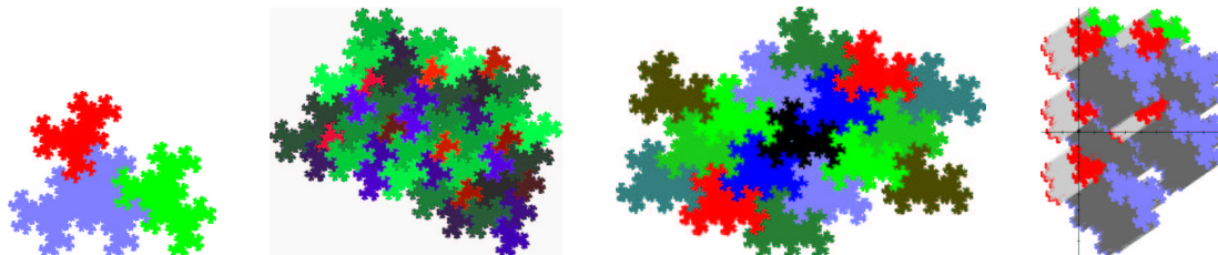
Figure 10: Central tile for the unimodular substitution of Pisot type 1 \rightarrow 12, 2 \rightarrow 3, 3 \rightarrow 1 . Self-replicating tiling, lattice tiling and Markov tiling. The associated Pisot number satisfies \beta^3 = \beta^2 + 1 . This substitution satisfies the numeration condition in [Sie04, Thu04] so that all multiple tilings are tilings.
