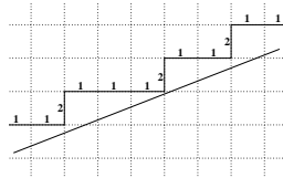
Fig. 1. The Sturmian sequence \dots 112111211211 \dots
