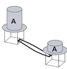
Fig. 7. Autoepistemic dialog
