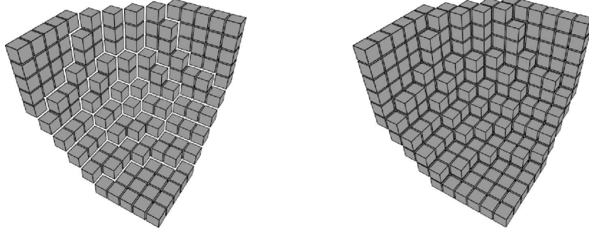
(a) Eighth of the naive discrete sphere. (b) Eighth of a standard discrete sphere.
