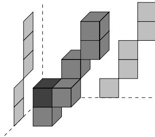
Fig. 2. The naive discrete line directed by (1, 2, 4) , for which projections are 2-dimensional naive discrete lines, contains an error in the point selection
