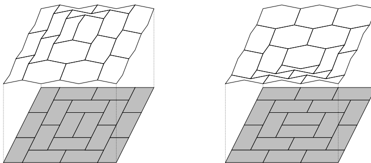
FIGURE 5. Patches of the pyramids \hat{h}_{v,z} (left) and \check{h}_{v,z} (right): domino tiling viewpoint (bottom) and lifted viewpoint (top). Note that the height is extremal in v in both cases.
