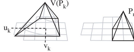
Figure 43: Simplification of V(P_k) .
