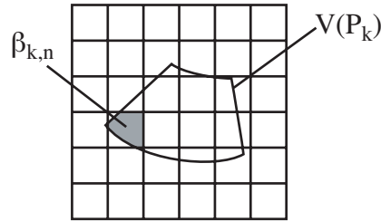
Figure 18: Probabilistic interaction using a uniform kernel.
