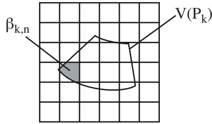
Figure 18: Probabilistic interaction using a uniform kernel.
