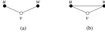
Fig. 5: Configurations of Properties 3.6 and 3.10.
