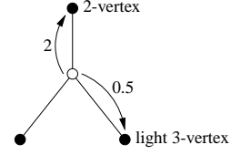
Fig. 12: Rule (R2.3)
