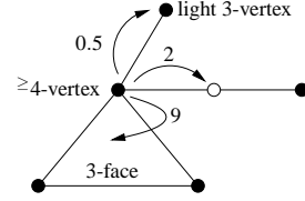
Fig. 9: Rule (R1)
