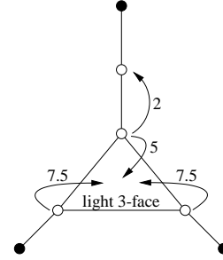
Fig. 10: Rule (R2.1)
